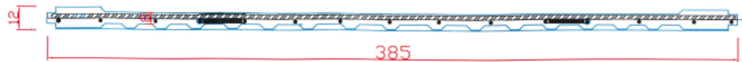
section B
